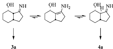
Scheme 4. Imine–enamine tautomeric equilibrium affording aldols 3a and 4a .
