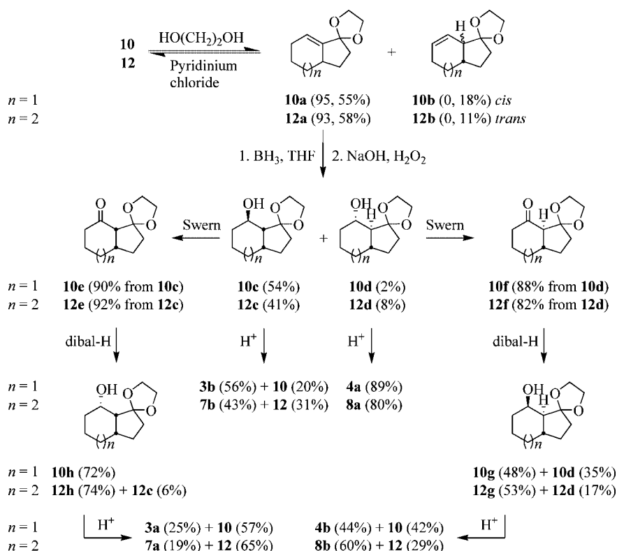
Scheme 5. Preparation of aldols 3 , 4 , 7 , and 8 .
