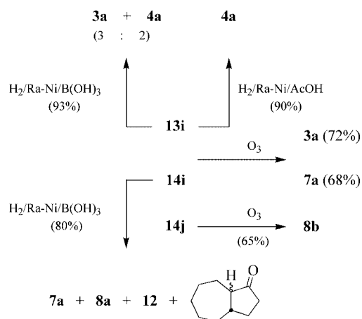
Scheme 3. Unmasking of isoxazolines 13i , 14i , and 14j to give aldols 3a , 4a , 7a , and 8 .
