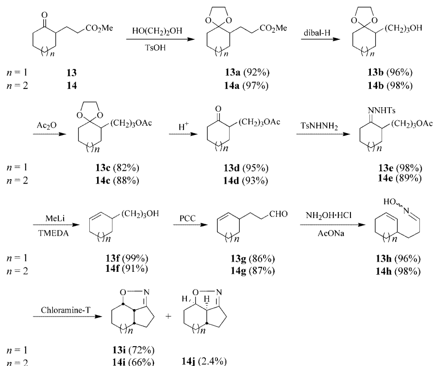
Scheme 2. Preparation of isoxazolines 13i , 14i , and 14j .
