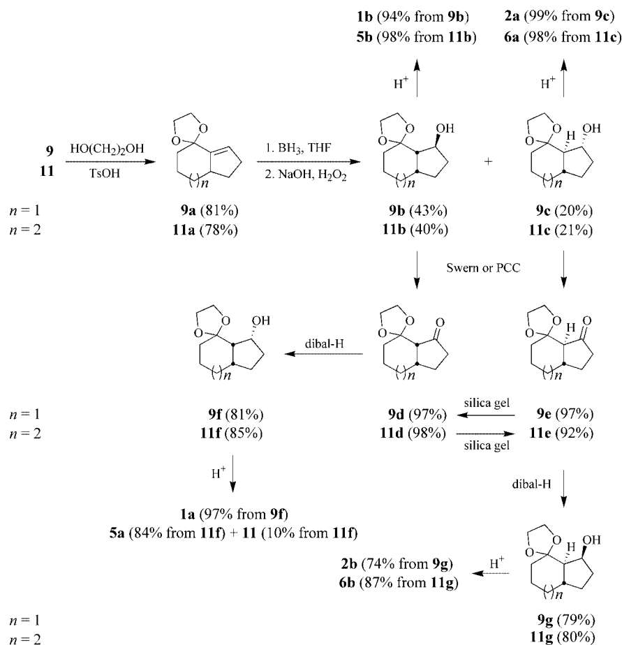
Scheme 1. Preparation of aldols 1 , 2 , 5 , and 6 .
