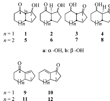
Figure 1. Hydroxyhydrindanones 1–4 , hydroxyhydroazulenones 5–8 , hydrindenones 9 , 10 , and hydroazulenones 11 , 12 .
